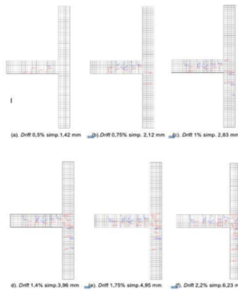
Figure 12. Pattern of monolithic beam-column (BN) joint cracks
