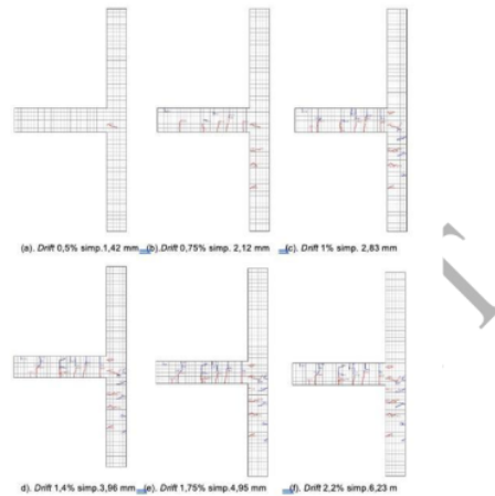
Figure 14. Crack pattern of 4-post precast beam-column connection (BG-2)
