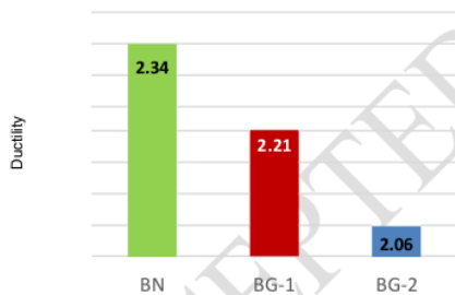
Figure 15. Ductility values for BN, BG-1, BG-2. Specimens
