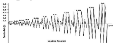
Figure 7. Loading program according to SNI 7834:2012
