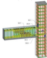
Figure 5. Strain gauge on steel
