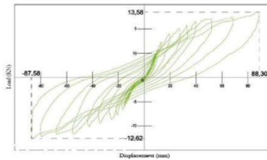
Figure 8. The load-displacement relationship due to cyclic loads on the BN test object
